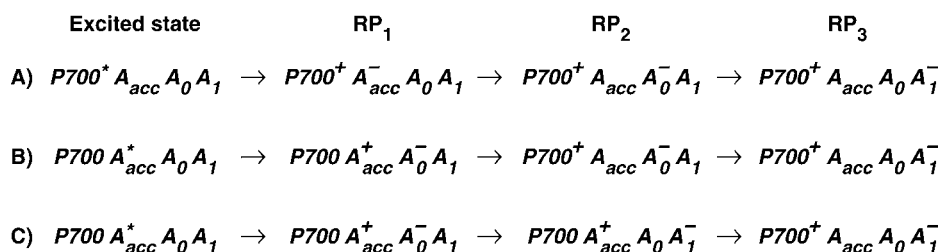
FIGURE 2 Three possible sequences of redox intermediates corresponding to the three radical pairs found in our previous work (8) (top). An alternative relaxed radical pair scheme with only two different redox intermediates is shown at the bottom. The latter scheme is not very likely, given the significant differences in the spectra of radical pairs RP2 and RP3. (Note that in Fig. 2 D, a relaxed radical pair scheme is shown containing two formally identical but energetically different RPs.) (Reproduced from Müller et al. (8).)
